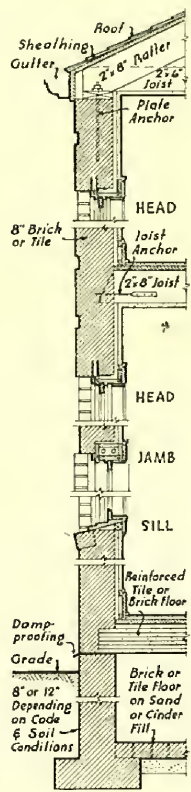
Wall Section
